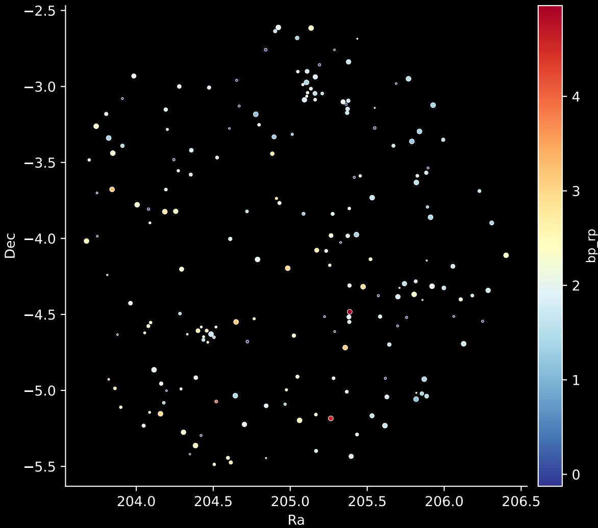
APOGEE DR17 Field: [218+00] Stars: 194
