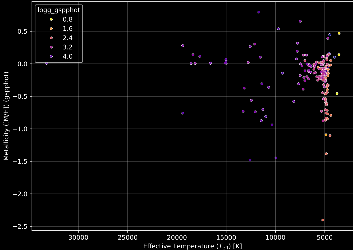
APOGEE DR17 Field: [218+00] Stellar Population Parameters (n= 194)
