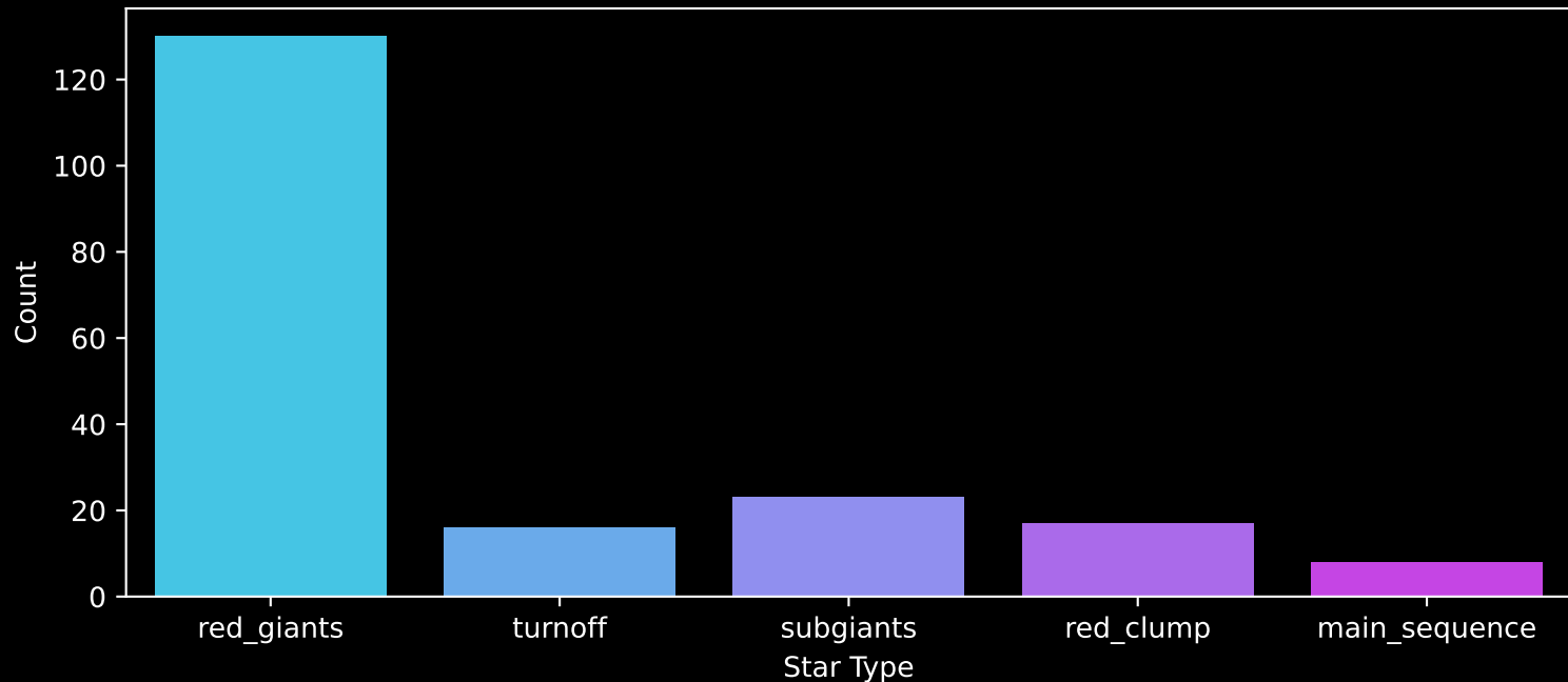
APOGEE DR17 Field: [218+00] Count plot of Star Type
