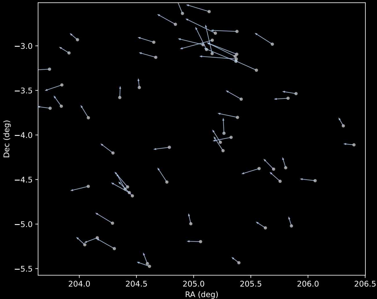
APOGEE DR17 Cluster 1 Proper Motion Vectors (n=60)
