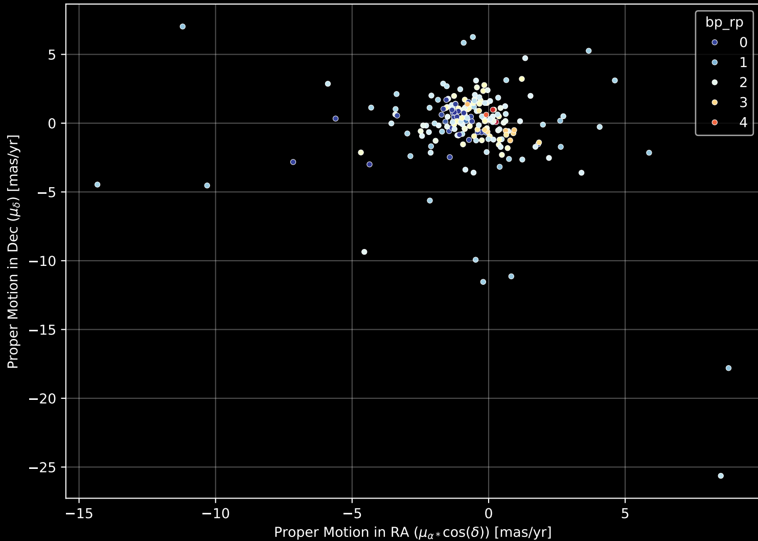
APOGEE DR17 Field: [218+00] Proper Motion Diagram (n= 194)
