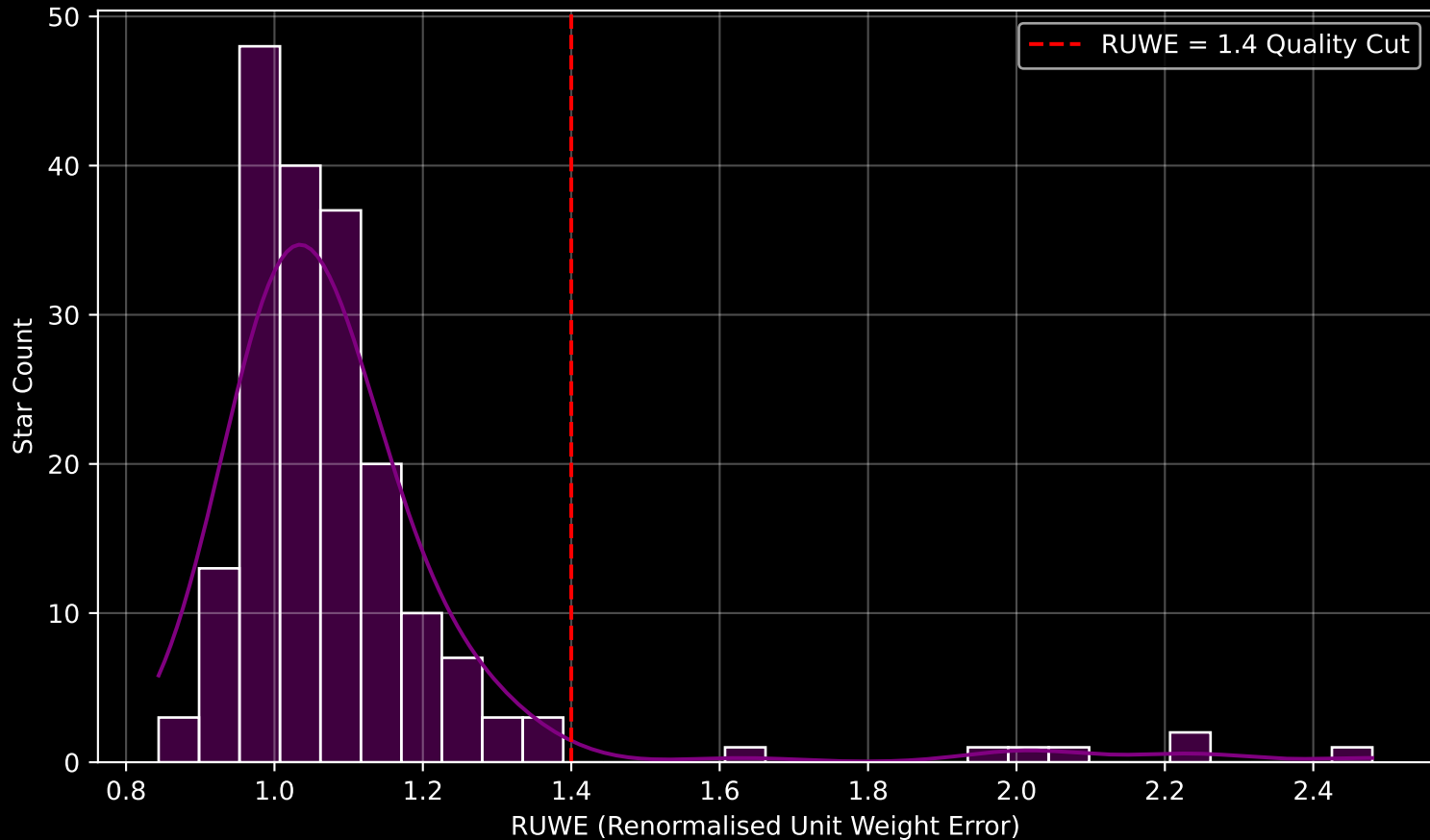
GAPOGEE DR17 Field [218+00] RUWE Distribution (n= 191)
