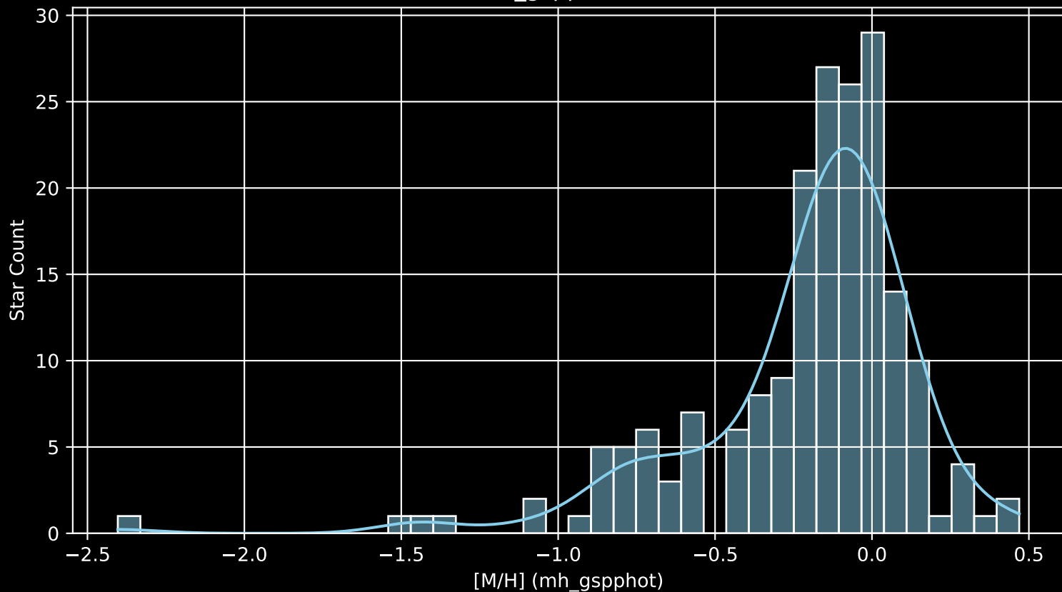
APOGEE DR17 Field: [218+00 [M/H] (mh_gspphot) (n= 191)
