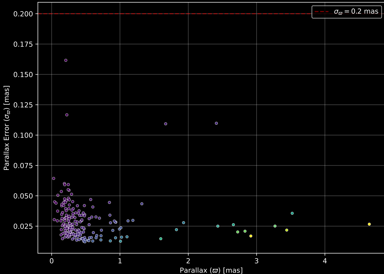
APOGEE DR17 Field: [218+00] Parallax Quality (n= 194)
